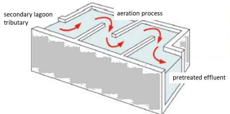
Figure 4 – Schematic of the contact tank adopted
