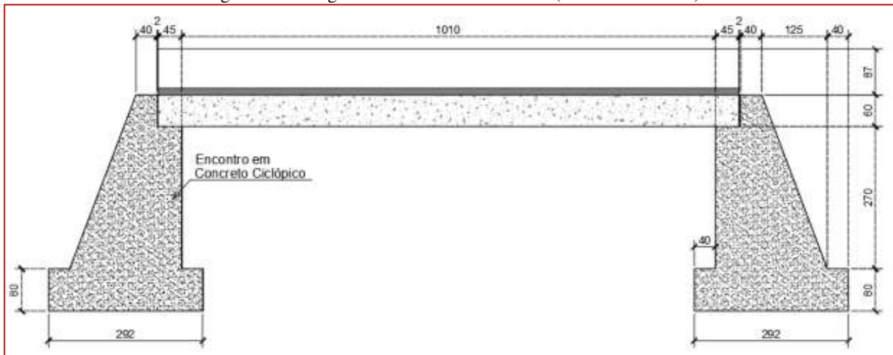
Figure 11 – Longitudinal section of the board (dimensions in cm).
