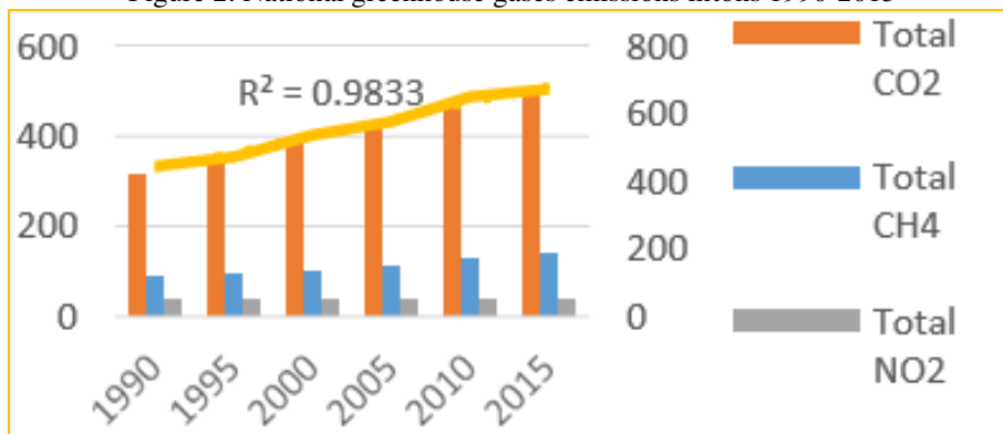
Figure 2. National greenhouse gases emissions intons 1990-2015
