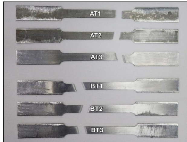
Figure 4 – Test specimens.
