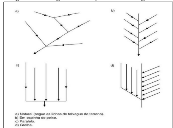
Figure 8. Configurations of possible drainage lines.
