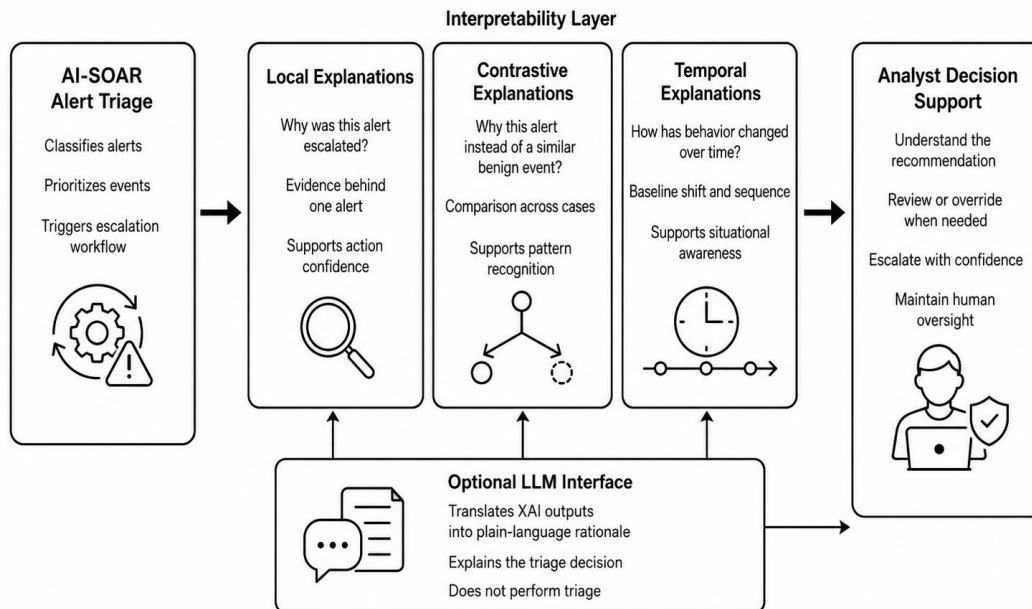
Figure 1. Three-Layer XAI Framework for Trust in AI-SOAR Escalation Workflows
