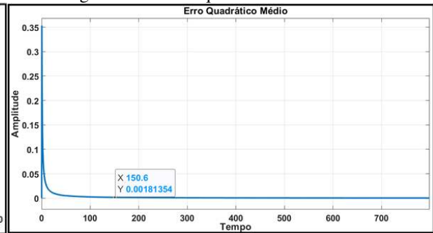
Figure 6 – Mean Squared Error for RLSM.
