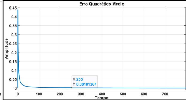
Figure 11 – Mean Squared Error for GM.
