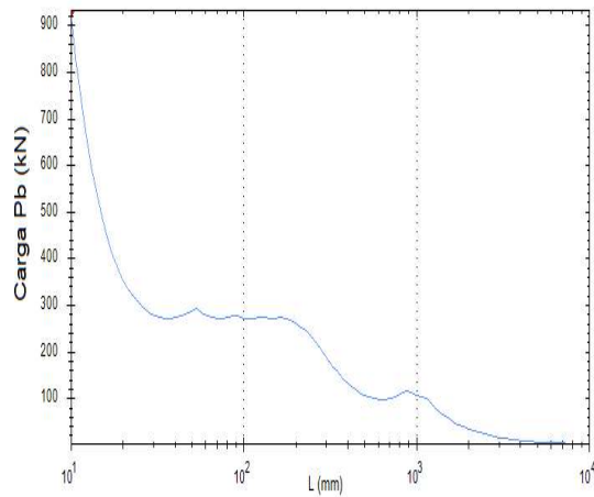
Figure 10: Z90 profile results with ribs in the soul and tables Curva Pb vs. L
