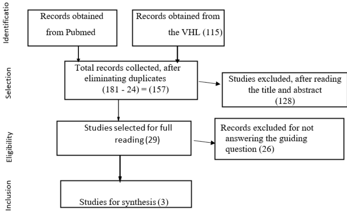
Figure 1 – PRISMA Flowchart
