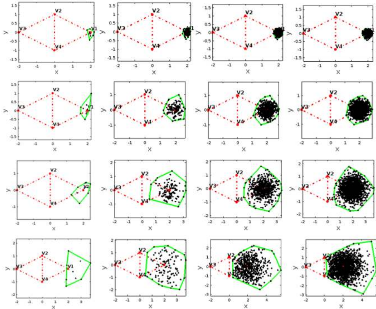
Figure 3 shows the points and convex closures that bound the constant topology region with different simulations, changing the value of \sigma to 0.1, 0.3, 0.5 e 1.0 ; each one with k = 10, 100, 500, 1000 . In the figure are shown in each line k = 10, 100, 500, 1000 para \sigma = 0.1 ; k = 10, 100, 500, 1000 to \sigma = 0.3 ; and so forth.
